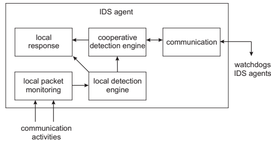
Fig. 3. The building blocks of the IDS client existing in each sensor node.
