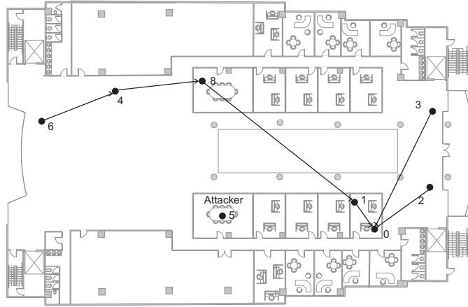
Fig. 6. The routing tree formed by the sensor nodes using MintRoute. Node 5 is the attacker launching a sinkhole attack.
