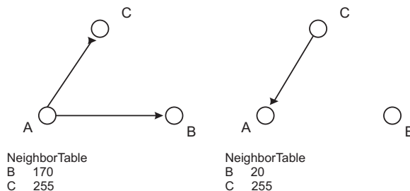
Fig. 2. The two phases of sinkhole attack. In the first phase node C (attacker) receives the route update packet of node A and in the second phase it sends the forged packet to A impersonating B .
